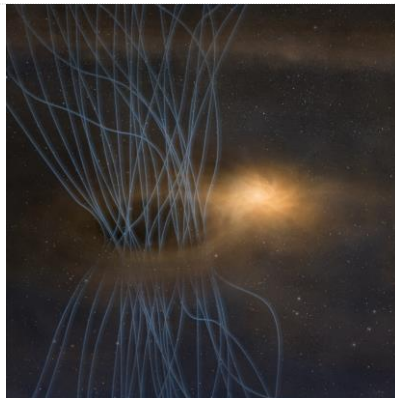
Fig. 1. Illustration of the 'sneeze' of magnetic flux from a baby star. The baby star at the center surrounded by a bright disk called a protostellar disk. Spikes of magnetic flux, gas, and dust in blue. Researchers found that the protostellar disk will expel magnetic flux, gas, and dust—much like a sneeze—during a star's formation.
